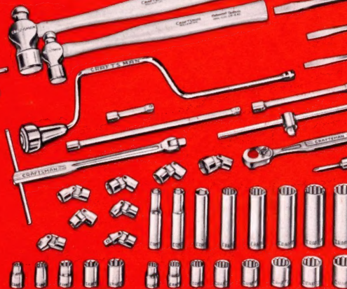
3/8-in. Square Drive Parts
